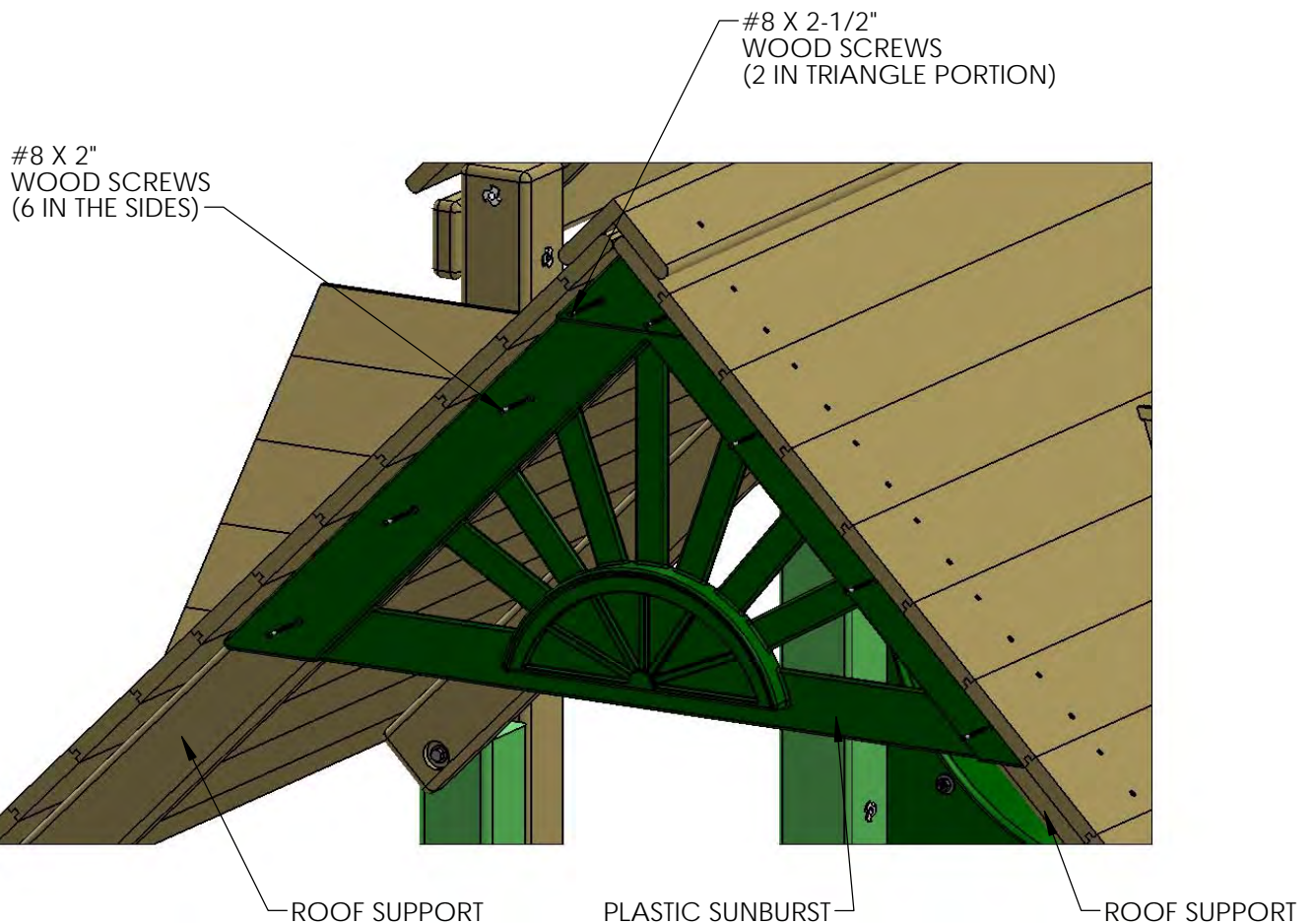
DETAIL A SCALE 1 : 8
