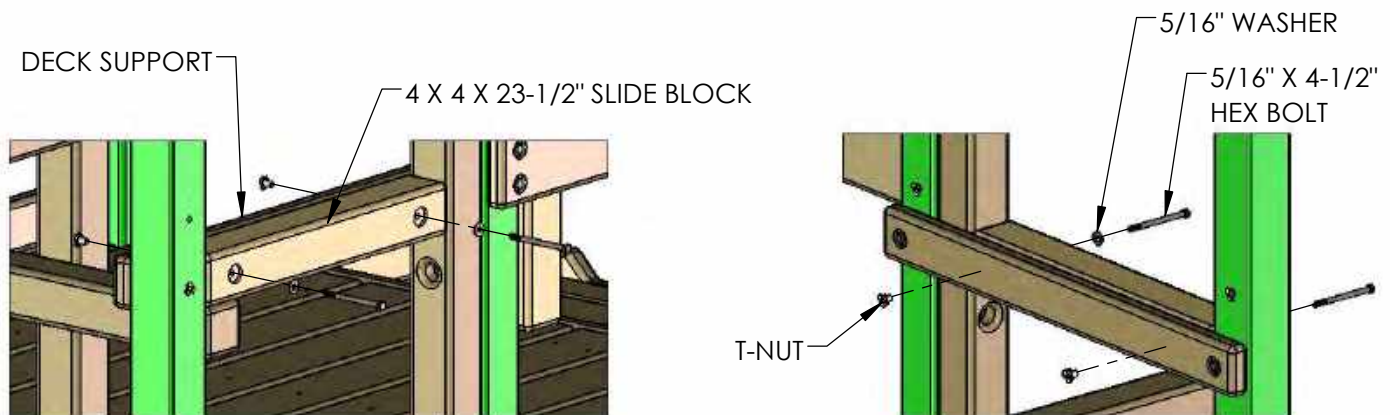
DETAIL A
