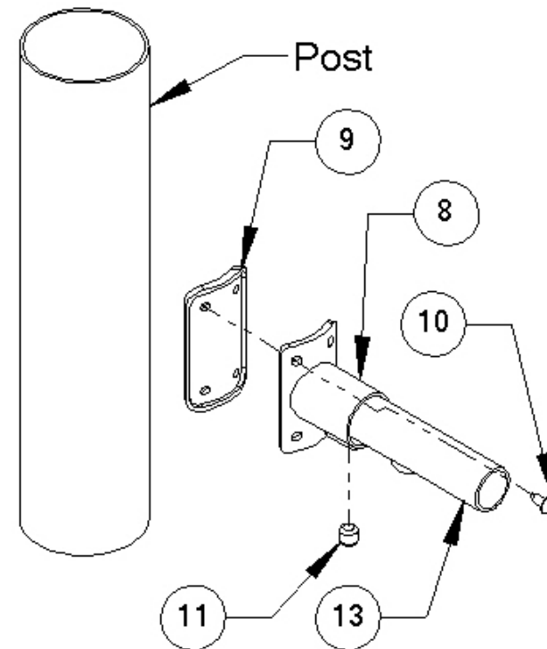
Detail A
