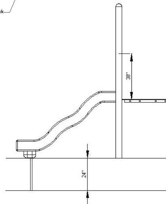
922-147 4' BUMP WAVE SLIDE FOOTING AND ELEVATION VIEW
