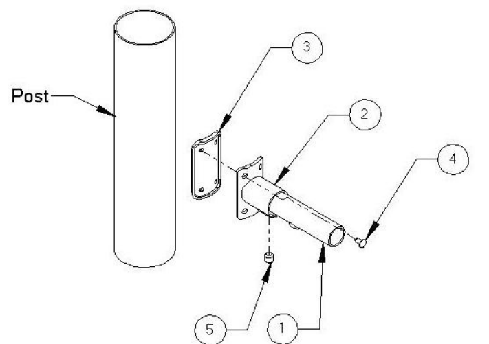
DETAIL C
