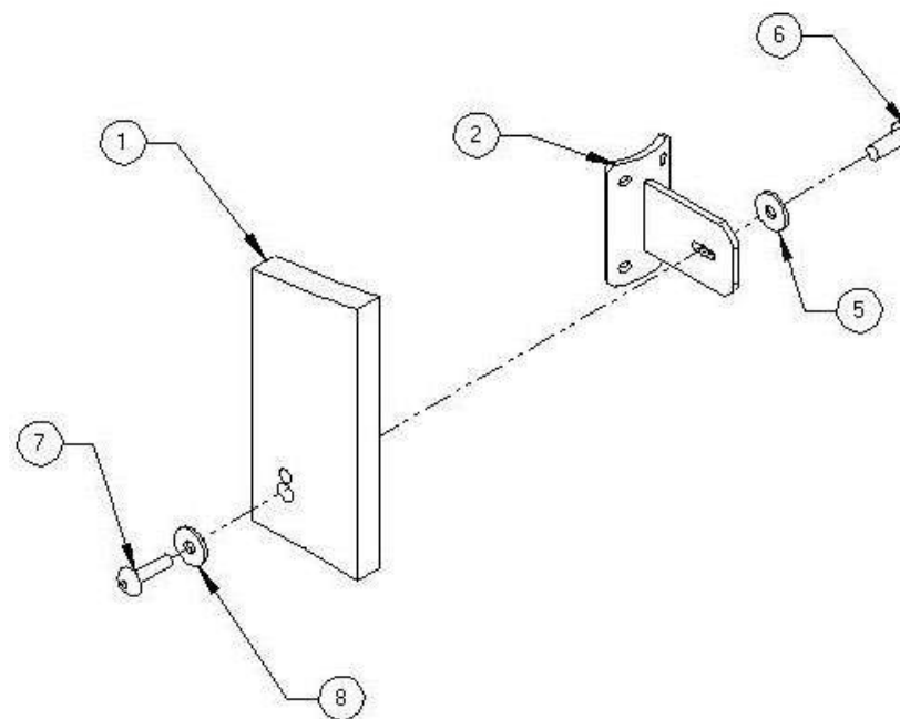
DETAIL B
