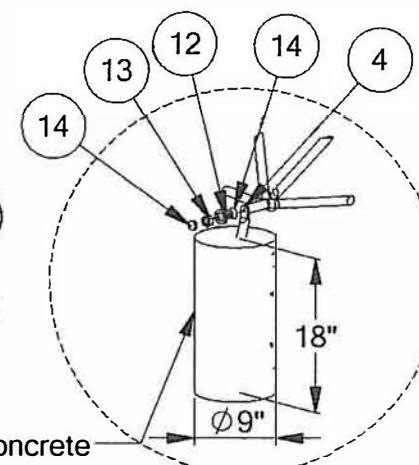
PERMANENT INSTALLATION
