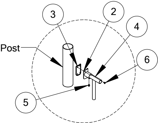
Detail A
