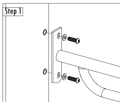
1" Button Cap Torx, Flat Washer (x4)
