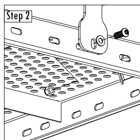
1" Button Cap Torx, Flat Washer, Locking Flange Nut (x4)
