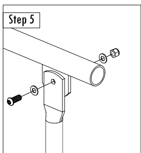
1" Button Cap Torx w/ Pin, Flat Washers, Lock Nut (x4)
