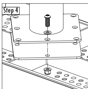
1" Button Cap Torx, Flat Washers, Locking Flange Nut (x8)
