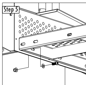
1" Button Cap Torx, Flat Washers, Locking Flange Nut (x2)
