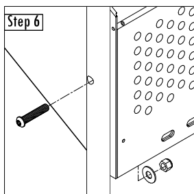
2" Button Cap Torx, Flat Washer, Lock Nut (x2)
