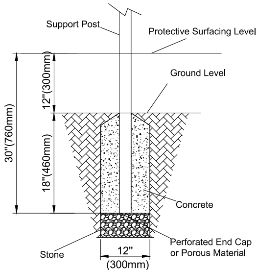
(DETAIL 3) Component Footing Detail
