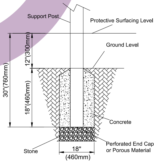
(DETAIL 1) Support Post Footing Detail
