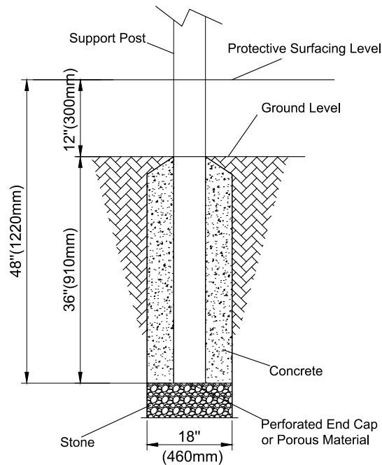
(DETAIL 2) Single Post Swing Footing Detail
