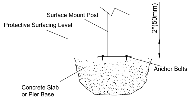
(DETAIL 4) Surface Mount Detail
